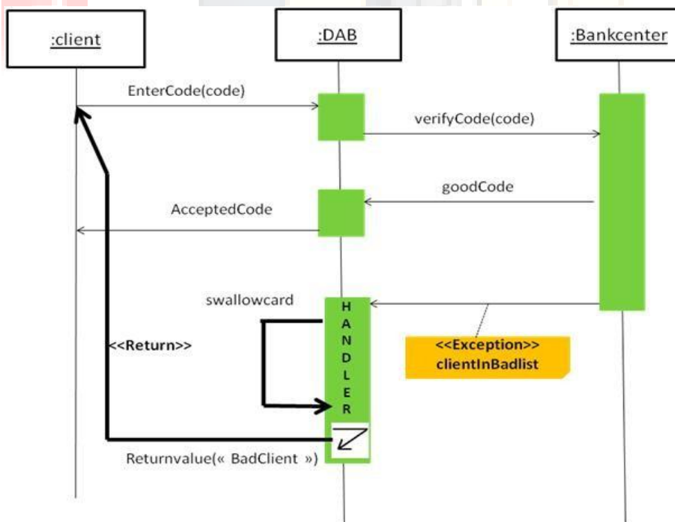
Figure 23: Application of return handling mode
