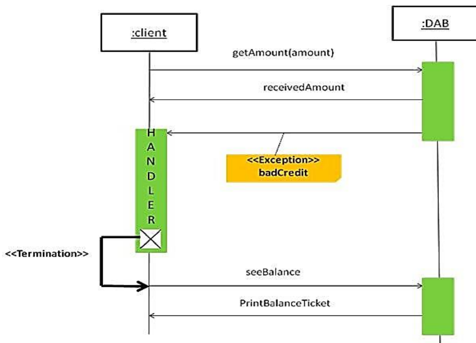
Figure 16: Application of termination handling mode
