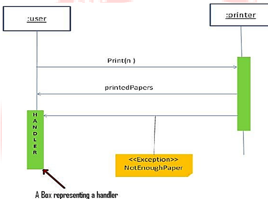
Figure 14: Use of Handler Stereotype
