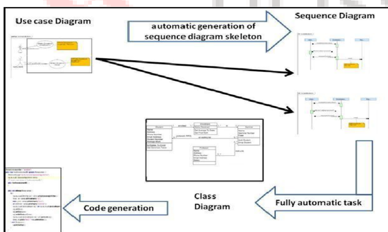
Figure 26: Main tasks of our proposed tool
