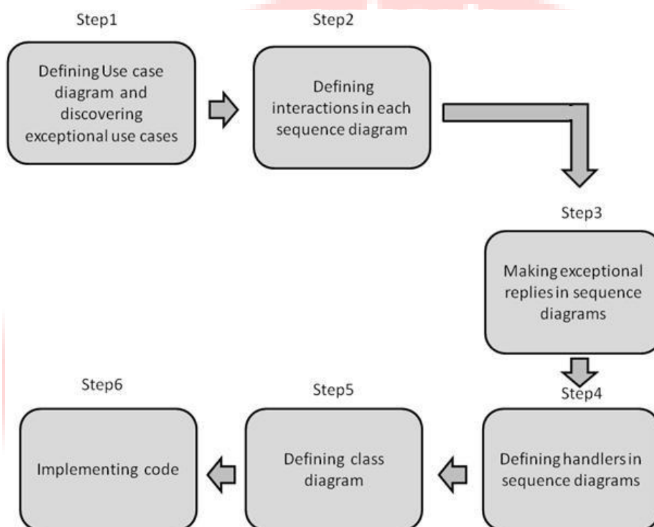
Figure 10: Process of our approach
