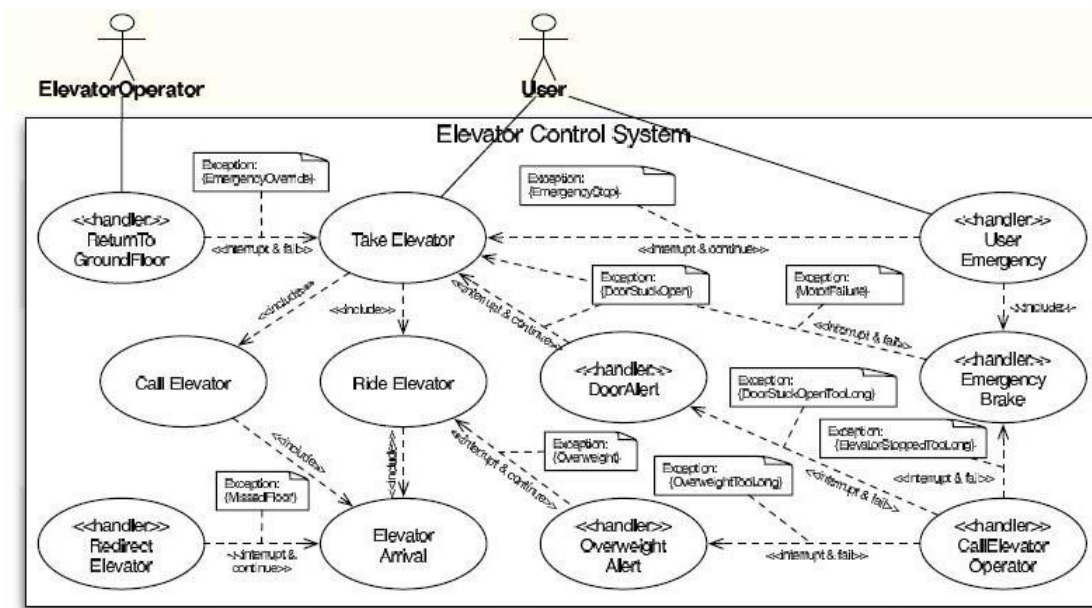
Figure 3: Exceptional Use Cases (extracted from [2])
