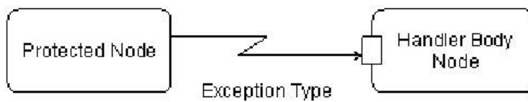
Figure 7: The UML 2.0 Exception Handling Notation (extracted from [UML Superstructure])
