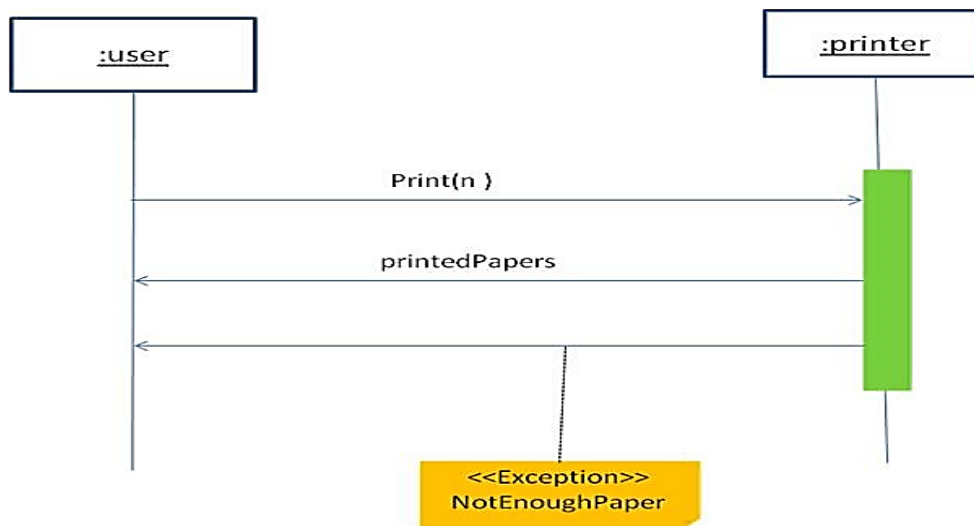
Figure 13: Example of sequence diagram after applying Exception stereotype
