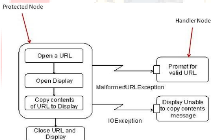
Figure 8: The URL viewer example (extracted from [UML Superstructure])
