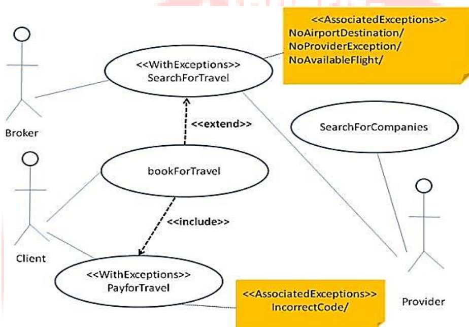
Figure 12: The travel agency use case diagram after applying the proposed stereotypes
