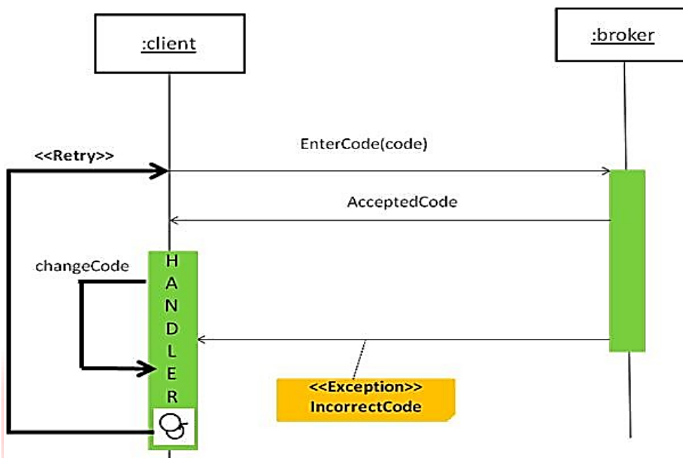
Figure 20: Application of retry handling mode
