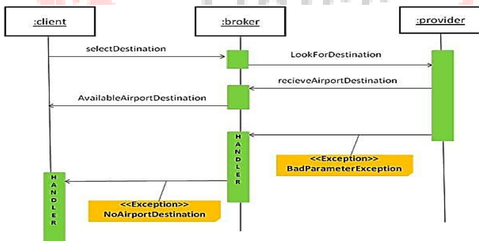
Figure 21: Application of resignaling handling mode
