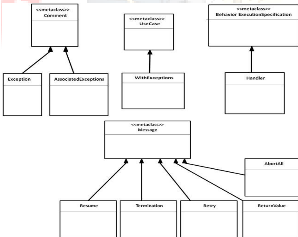
Figure 9: Exception Handling Profile
